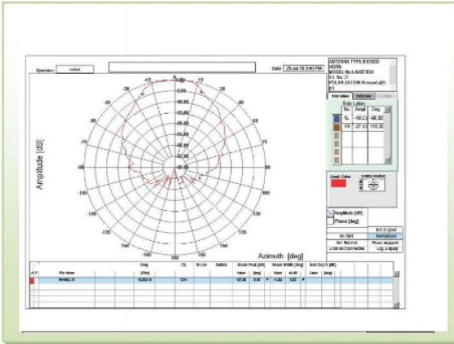
Radiation pattern
