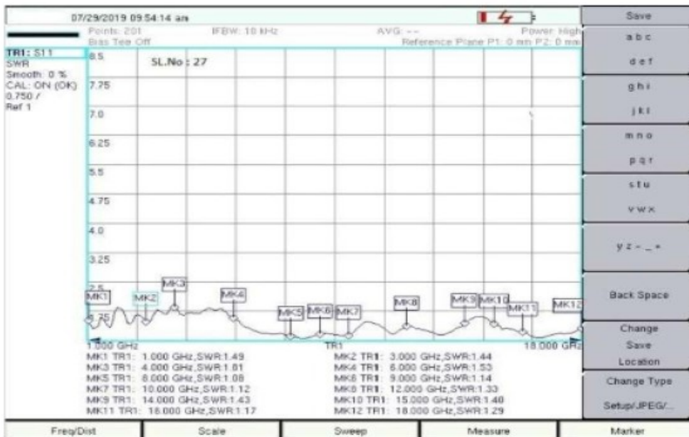
VSWR Plot
