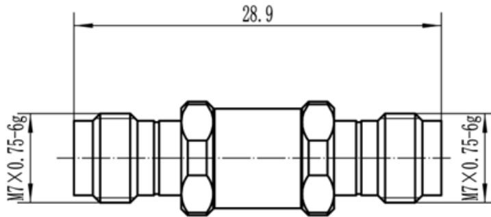
Drawing(mm)
